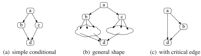
Figure 11. Recognizing conditionals
