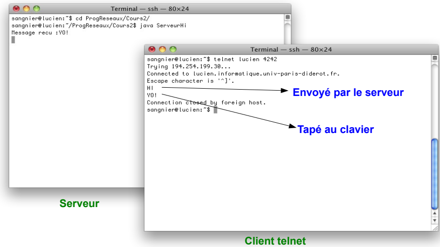
Client telnet
