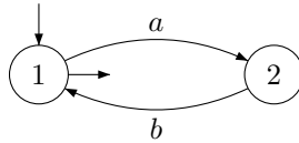
Figure 3: The minimal automaton of (ab)^* .
