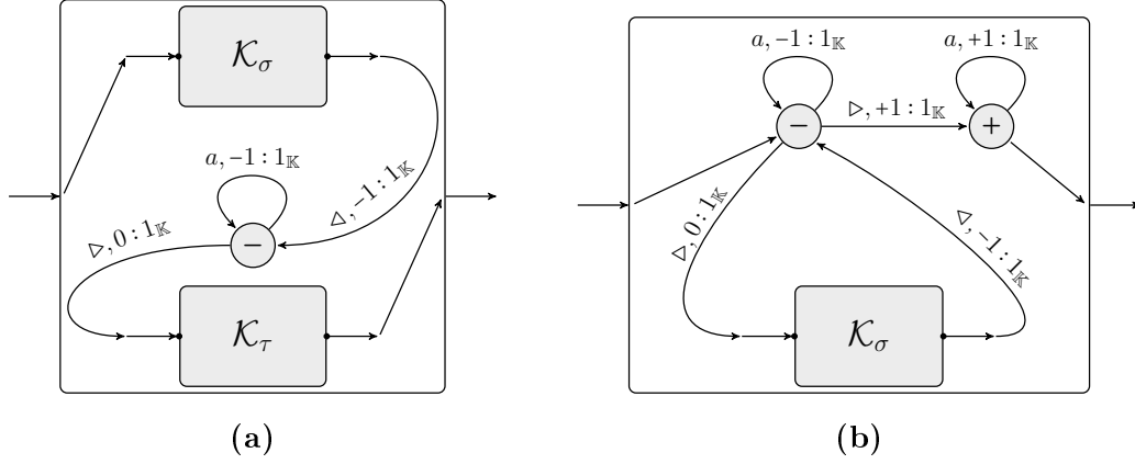
FIGURE 4.1 – Construction of transducers accepting \sigma \hat{\oplus} \tau (a) and \sigma^{\oplus} (b) respectively.
