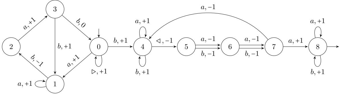
FIGURE 2.1 – The graphical representation of the FA \mathcal{A} given in Example 2. The state of the FA are the vertices while each transition (q, a, d, q') is depicted as an edge from q to q' labelled by a, d . The initial and accepting states are denoted by an incoming and an outgoing arrow respectively.
