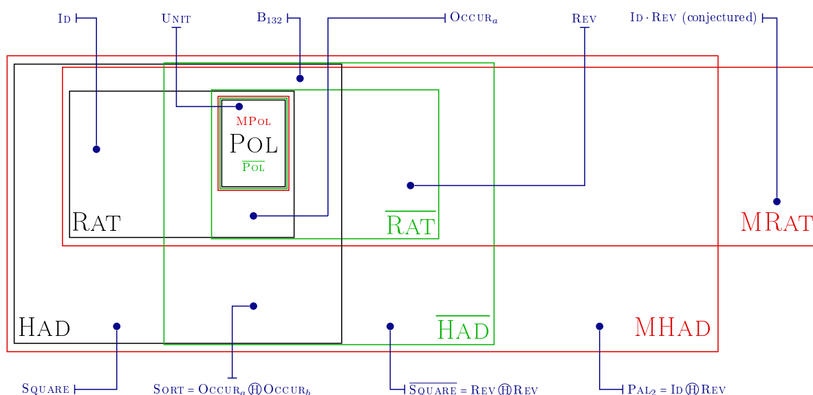
FIGURE 4.6 – The Hadamard hierarchy
