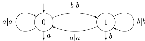
Figure 3: A subsequential transducer.
