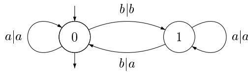
Figure 2: A sequential transducer.
