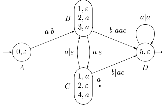
Figure 5: Determinization of the transducer of Figure 4
