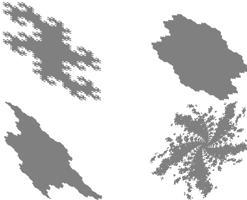
FIGURE 1. Examples of SRS tiles: The upper left tile is the so-called twin dragon fractal ( cf. [26]), right beside it is the well-known Rauzy fractal associated with the Tribonacci number ( cf. [34]). The lower left tile is known as “Hokkaido fractal” and corresponds to the smallest Pisot number which has minimal polynomial x^3 - x - 1 ( cf. [3]). The lower right one seems to be new, and is an SRS tile associated with the parameter \mathbf{r} = (9/10, -11/20) .
