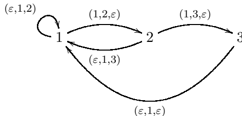
FIGURE 4.1. The prefix-suffix automaton for the Tribonacci substitution
