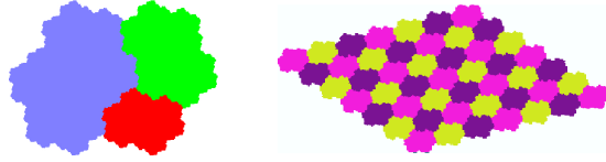
FIGURE 4.3. Rauzy fractal for the Tribonacci substitution, and Rauzy lattice tiling
