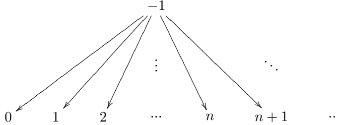
FIGURE 5.3. The hedgehog tree
