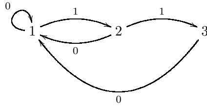
FIGURE 4.2. The prefix-suffix automaton recognizing the \beta -shift for the Tribonacci number
