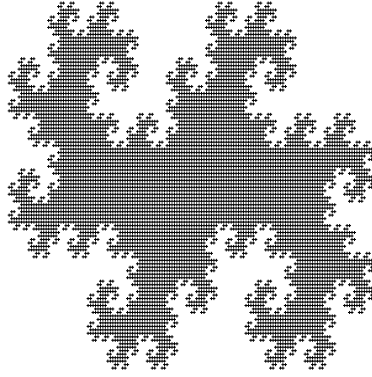
FIGURE 3.2. Knuth's twin dragon
