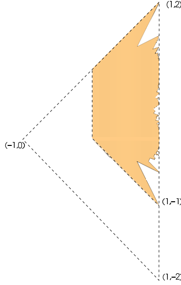
FIGURE 3.1. An approximation of \mathcal{D}_2^0
